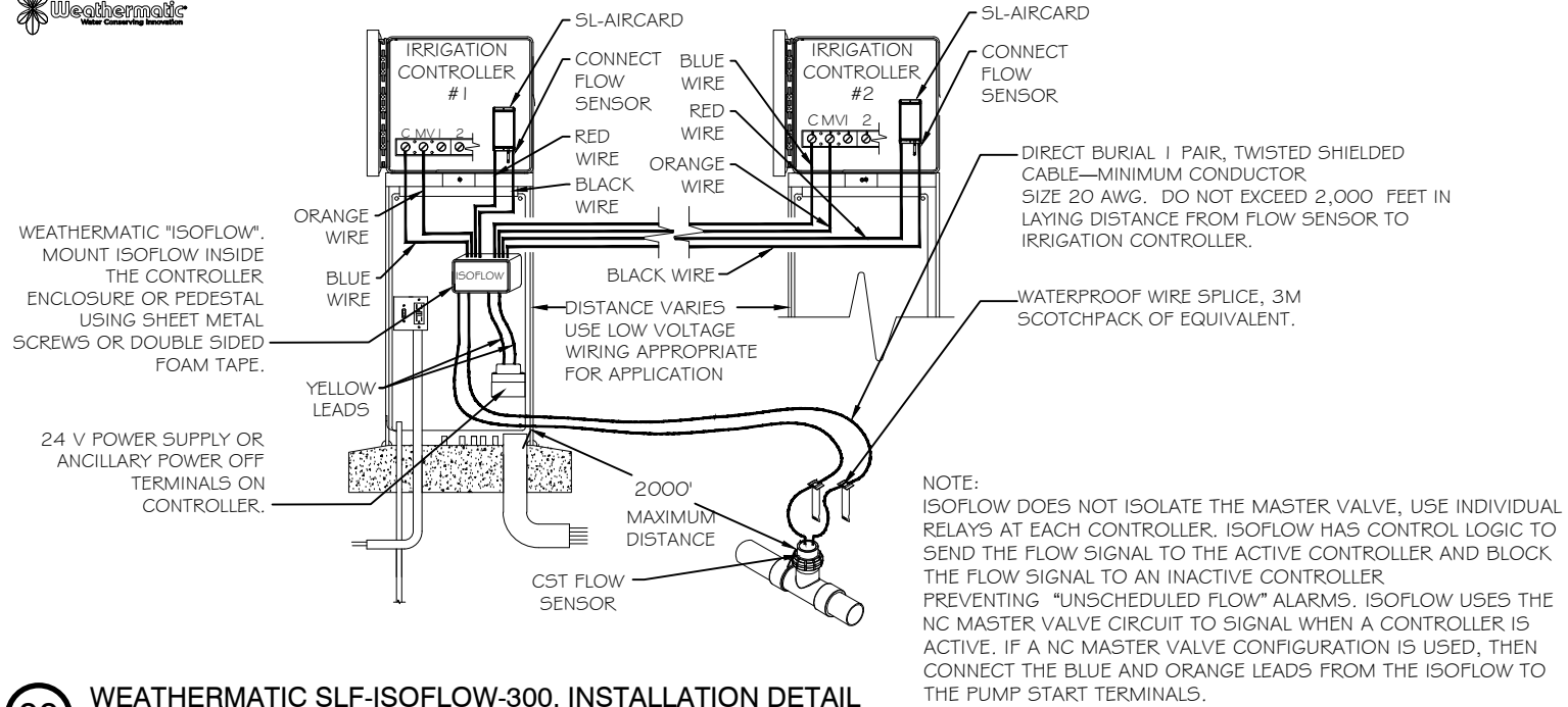
00 WEATHERMATIC SLF-ISOFLOW-300, INSTALLATION DETAIL NTS
